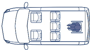
Standard 'Bench' conversion retains the original Ford seats with one wheelchair position.
